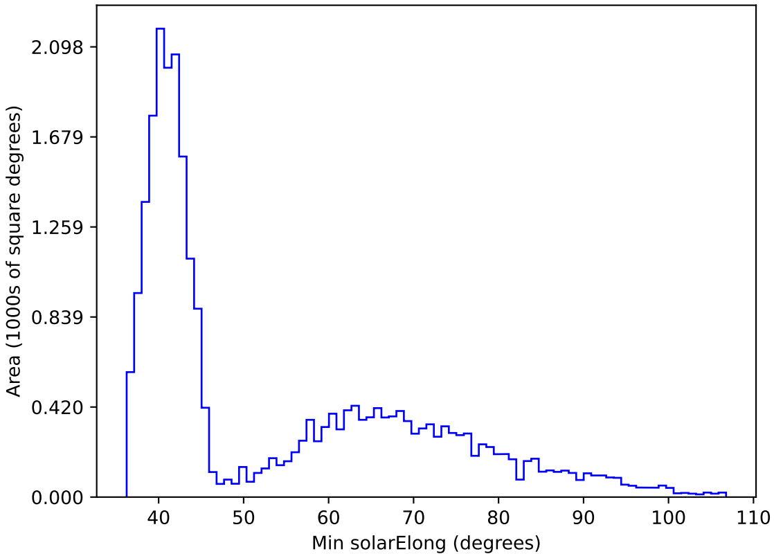
too_elab_r256_d2_griz_v3.4_10yrs All sky z band: Min solarElong
