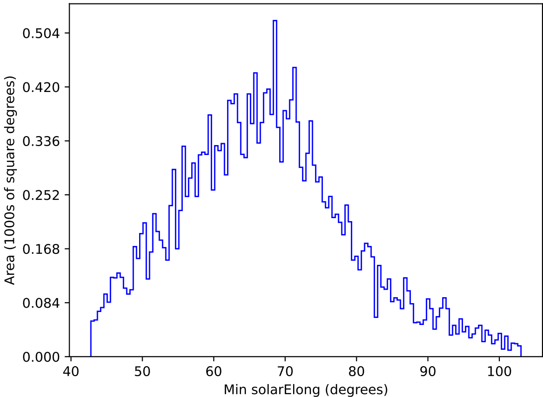
too_elab_r256_d2_griz_v3.4_10yrs All sky y band: Min solarElong
