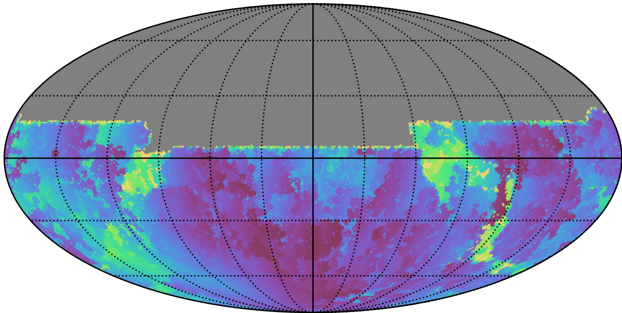
too_elab_r256_d2_griz_v3.4_10yrs All sky u band: Min solarElong
