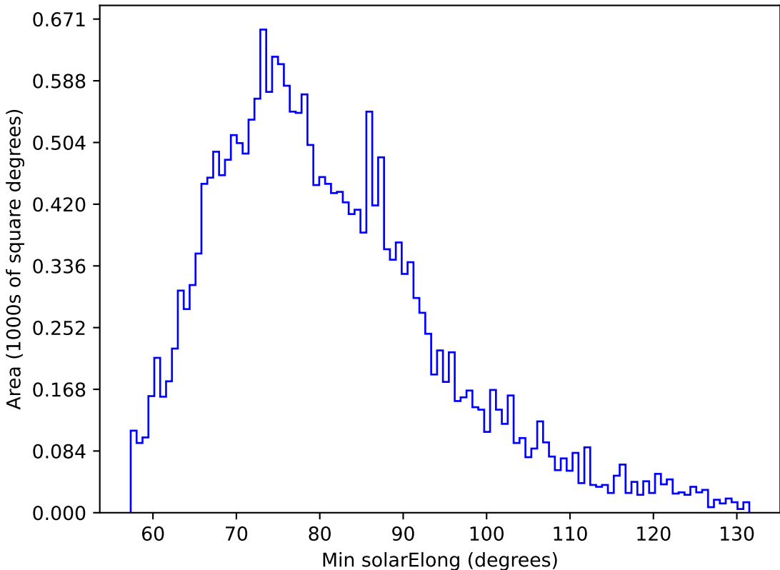
too_elab_r256_d2_griz_v3.4_10yrs All sky u band: Min solarElong
