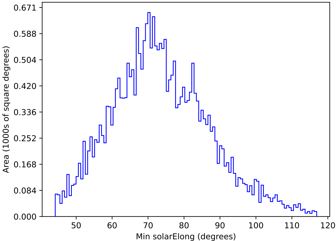
too_elab_r256_d2_griz_v3.4_10yrs All sky g band: Min solarElong
