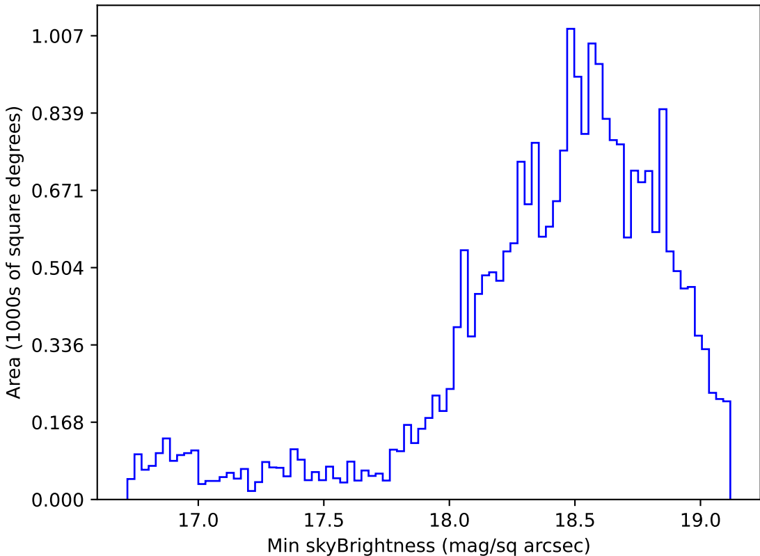
too_elab_r256_d2_griz_v3.4_10yrs Yr 1 z band: Min skyBrightness
