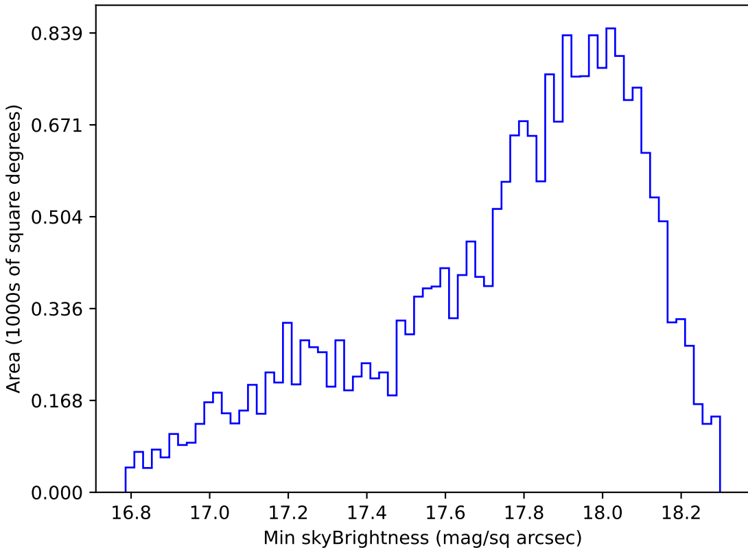
too_elab_r256_d2_griz_v3.4_10yrs Yr 1 y band: Min skyBrightness
