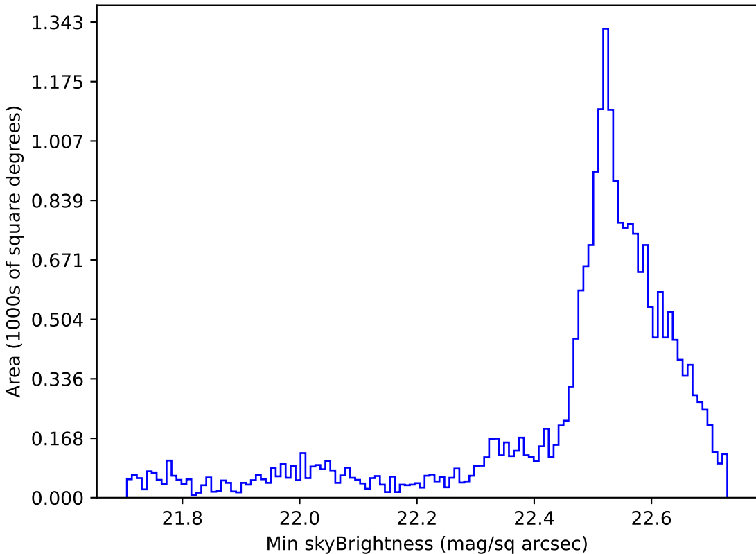
too_elab_r256_d2_griz_v3.4_10yrs Yr 1 u band: Min skyBrightness
