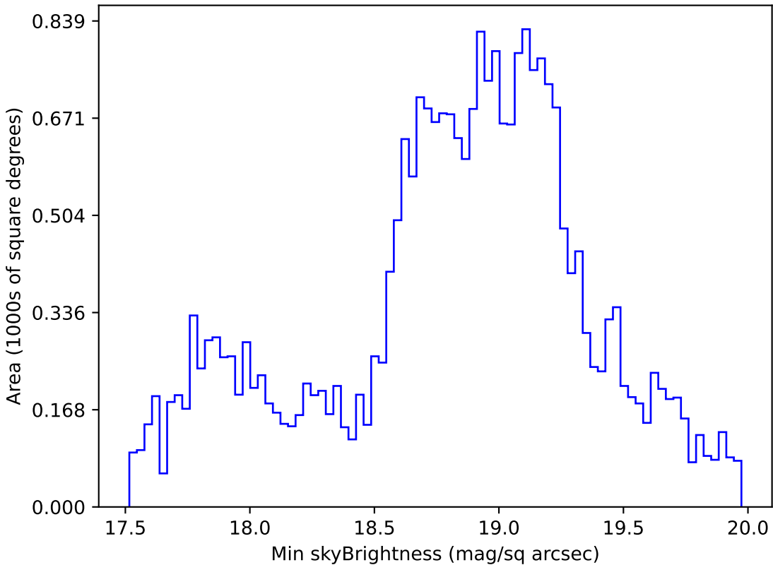
too_elab_r256_d2_griz_v3.4_10yrs Yr 1 i band: Min skyBrightness
