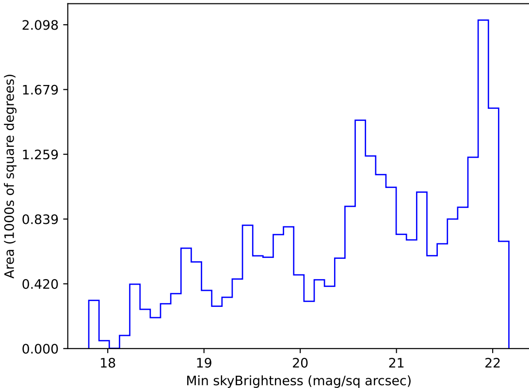
too_elab_r256_d2_griz_v3.4_10yrs Yr 1 g band: Min skyBrightness
