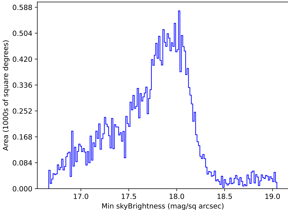
too_elab_r256_d2_griz_v3.4_10yrs Yr 1 all bands: Min skyBrightness
