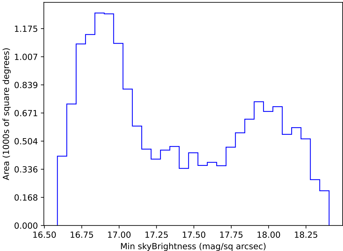
too_elab_r256_d2_griz_v3.4_10yrs WFD z band: Min skyBrightness
