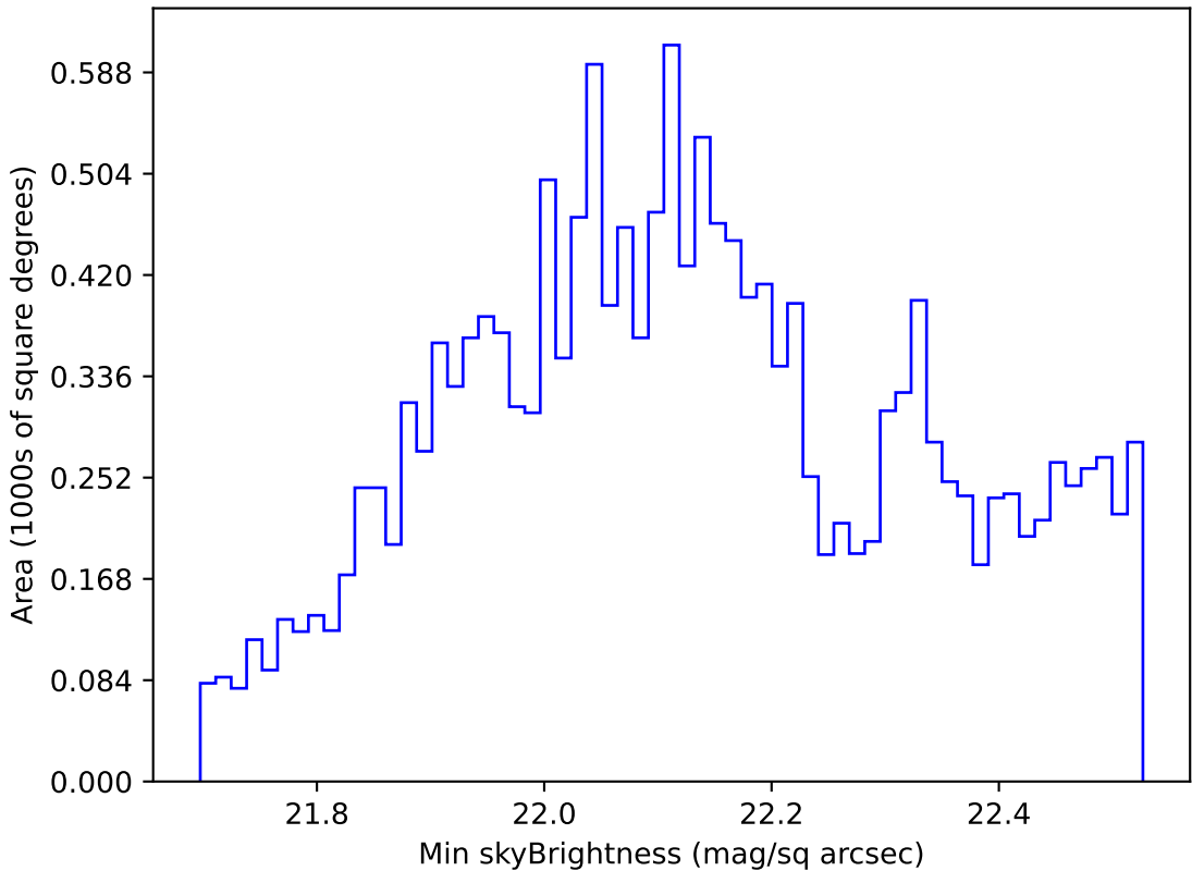
too_elab_r256_d2_griz_v3.4_10yrs WFD u band: Min skyBrightness
