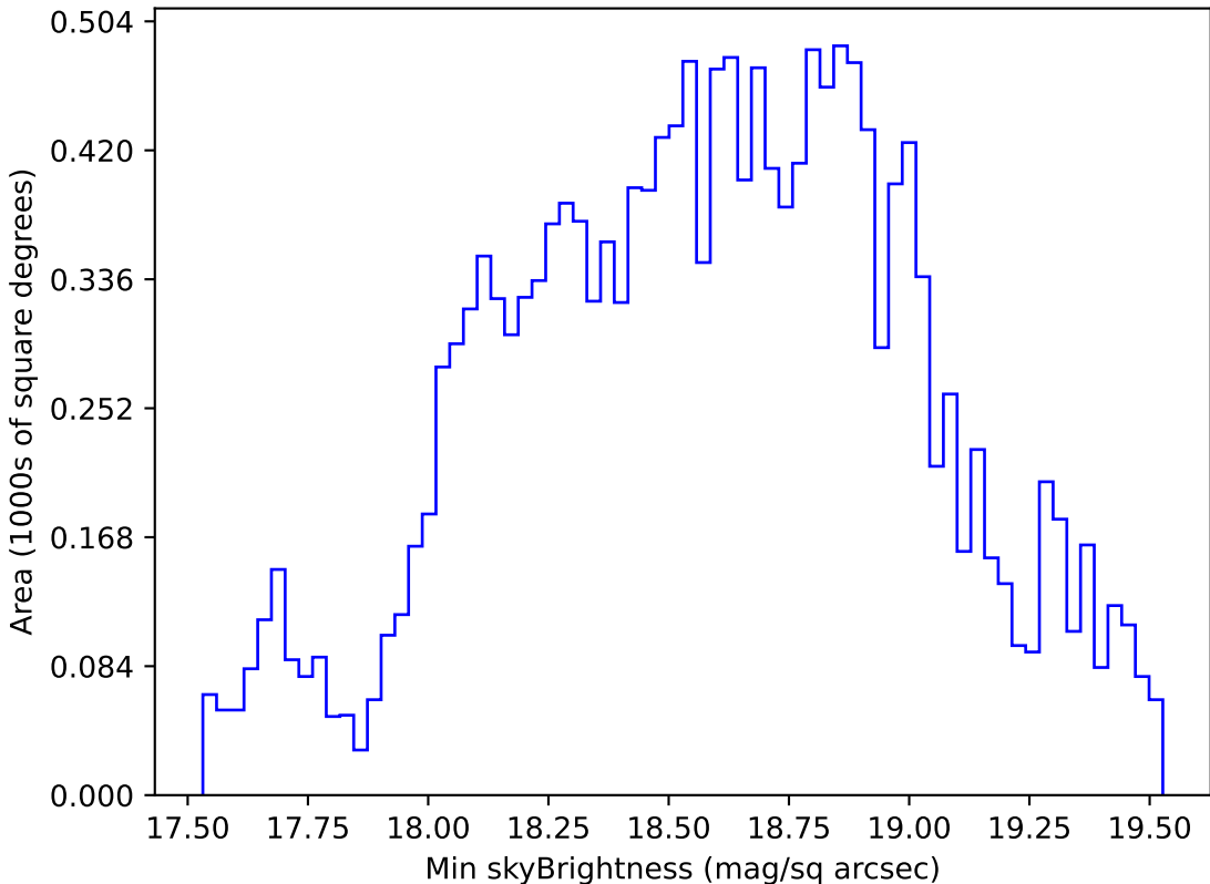
too_elab_r256_d2_griz_v3.4_10yrs WFD r band: Min skyBrightness
