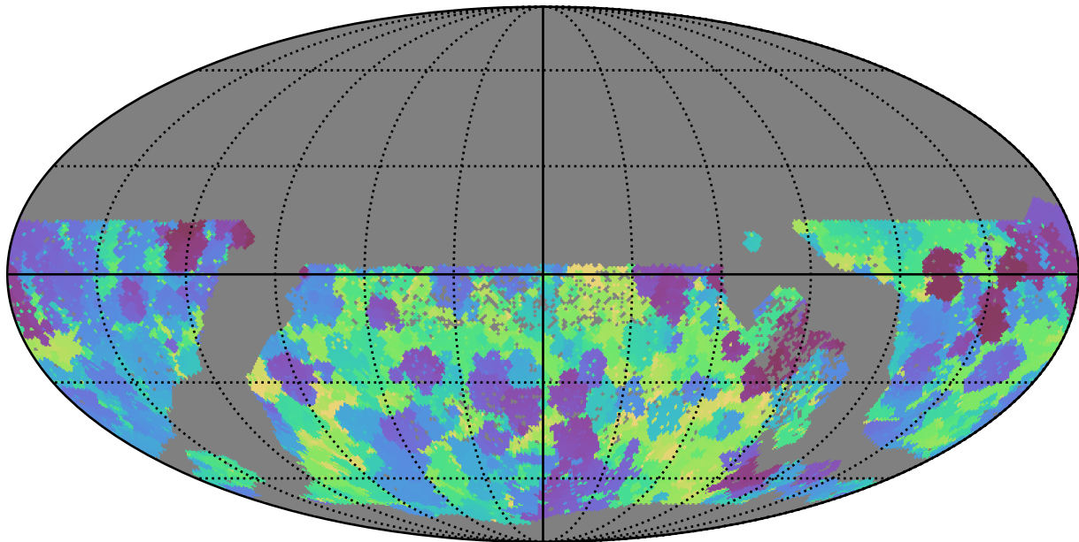
too_elab_r256_d2_griz_v3.4_10yrs WFD g band: Min skyBrightness
