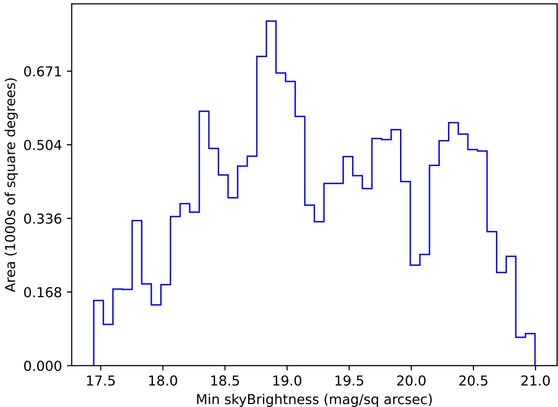
too_elab_r256_d2_griz_v3.4_10yrs WFD g band: Min skyBrightness
