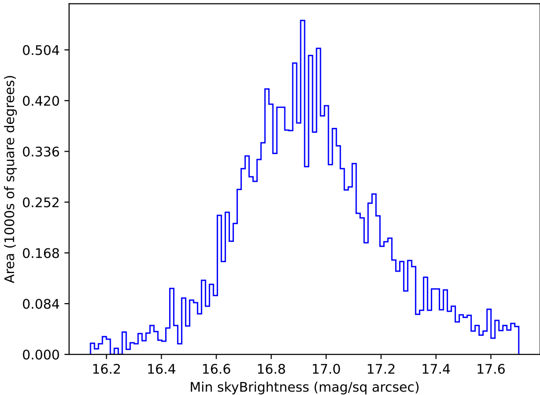
too_elab_r256_d2_griz_v3.4_10yrs WFD all bands: Min skyBrightness
