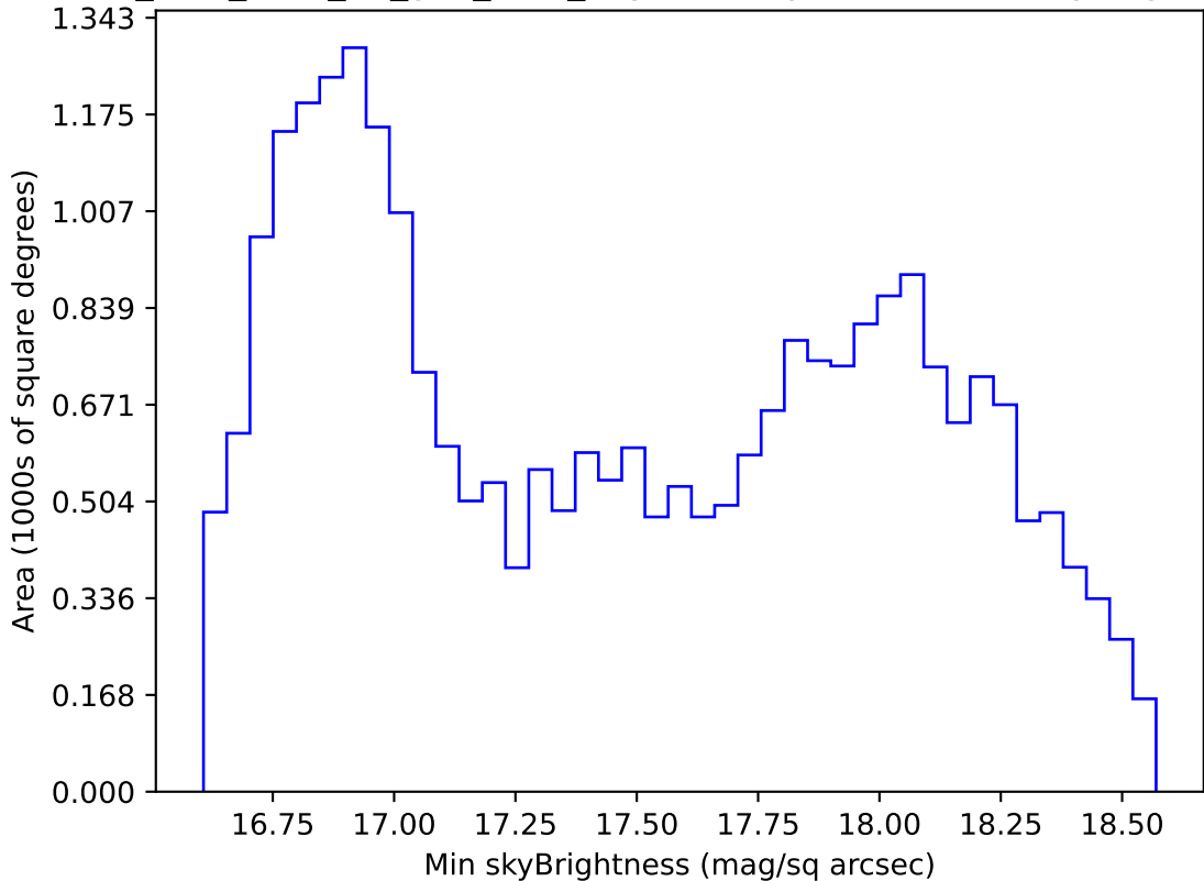
too_elab_r256_d2_griz_v3.4_10yrs All sky z band: Min skyBrightness
