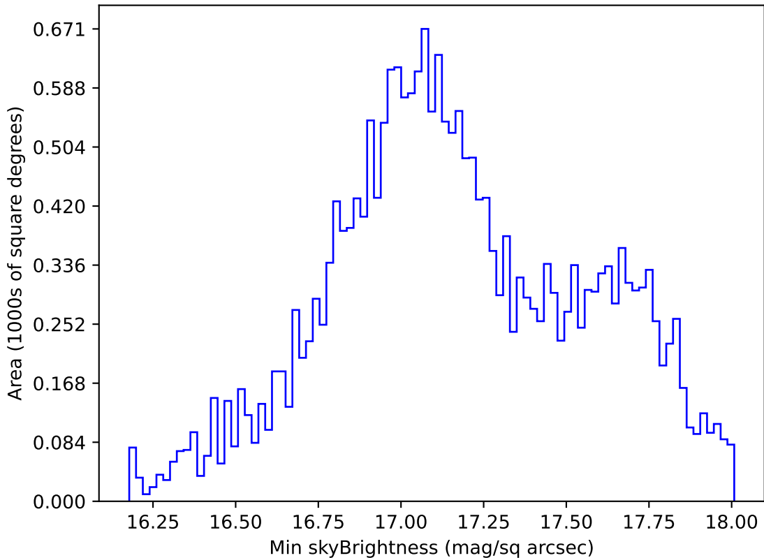
too_elab_r256_d2_griz_v3.4_10yrs All sky y band: Min skyBrightness
