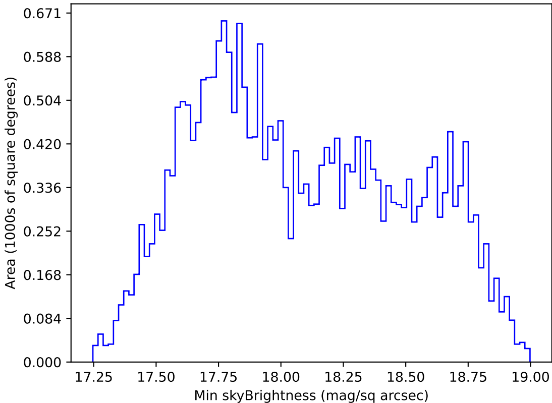
too_elab_r256_d2_griz_v3.4_10yrs All sky i band: Min skyBrightness
