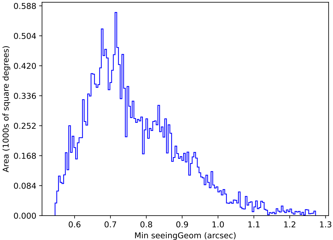
too_elab_r256_d2_griz_v3.4_10yrs Yr 1 u band: Min seeingGeom
