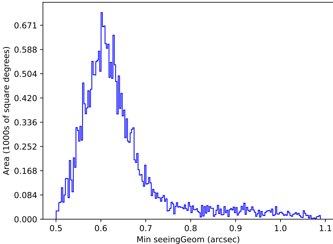
too_elab_r256_d2_griz_v3.4_10yrs Yr 1 r band: Min seeingGeom
