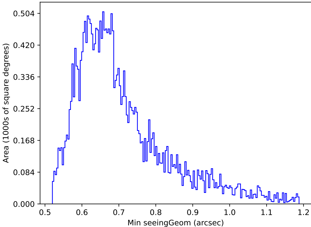
too_elab_r256_d2_griz_v3.4_10yrs Yr 1 g band: Min seeingGeom
