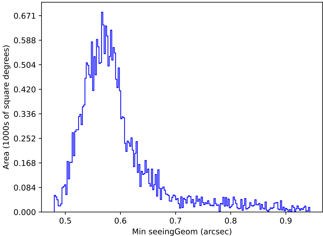
too_elab_r256_d2_griz_v3.4_10yrs Yr 1 all bands: Min seeingGeom
