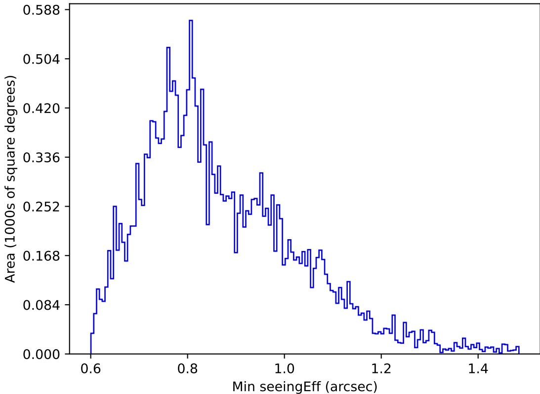
too_elab_r256_d2_griz_v3.4_10yrs Yr 1 u band: Min seeingEff
