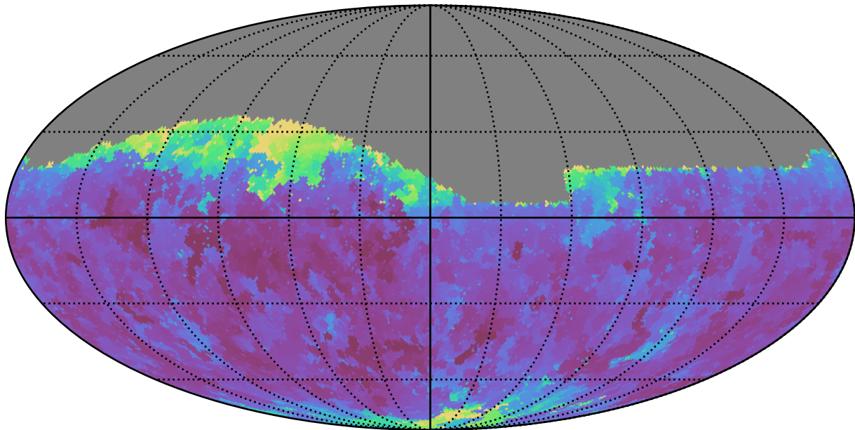
too_elab_r256_d2_griz_v3.4_10yrs Yr 1 r band: Min seeingEff
