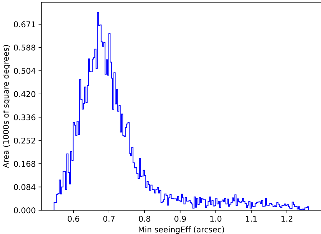
too_elab_r256_d2_griz_v3.4_10yrs Yr 1 r band: Min seeingEff
