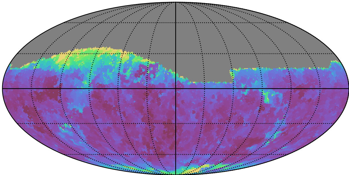
too_elab_r256_d2_griz_v3.4_10yrs Yr 1 i band: Min seeingEff
