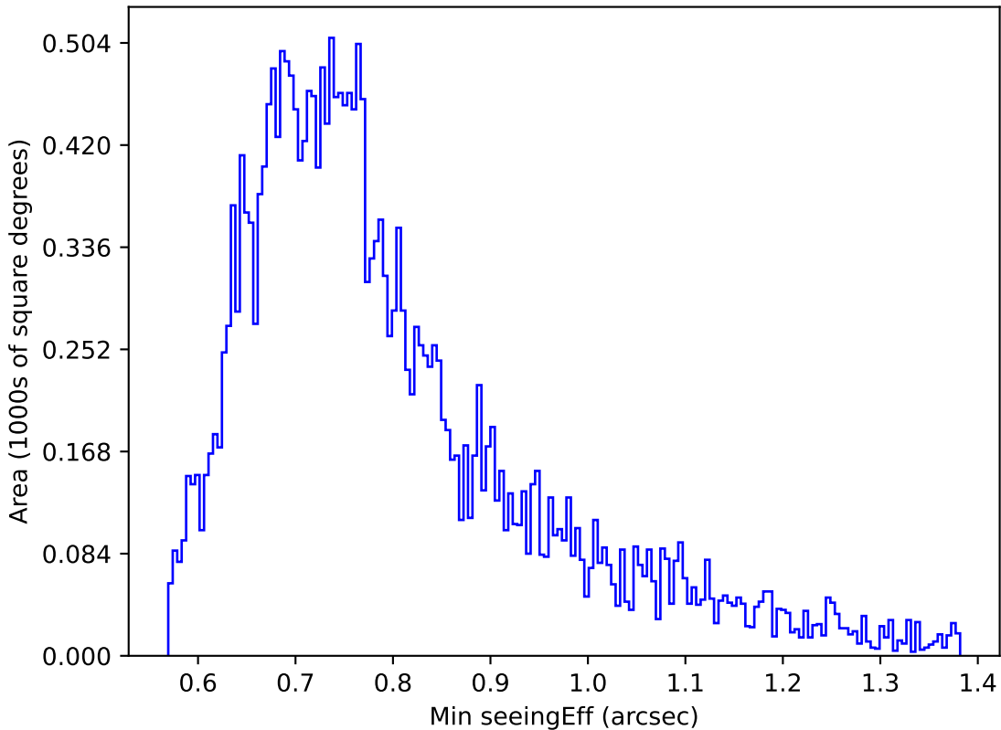
too_elab_r256_d2_griz_v3.4_10yrs Yr 1 g band: Min seeingEff
