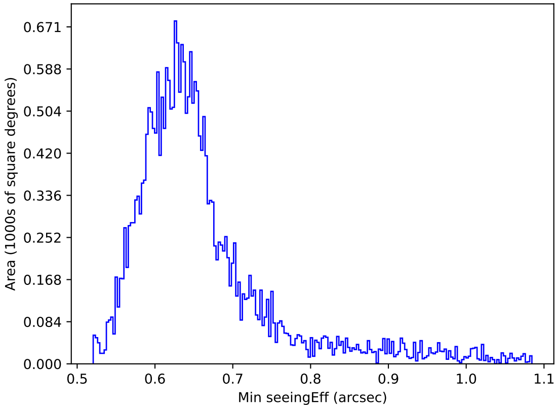
too_elab_r256_d2_griz_v3.4_10yrs Yr 1 all bands: Min seeingEff
