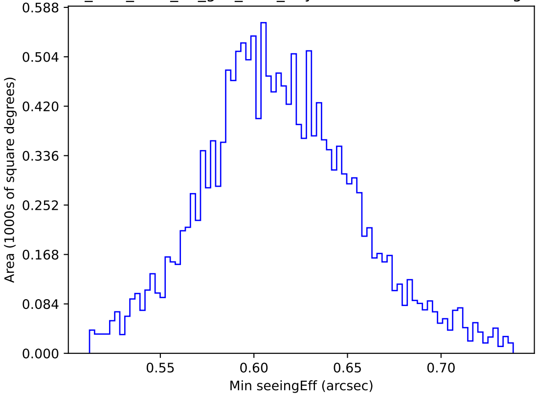
too_elab_r256_d2_griz_v3.4_10yrs WFD z band: Min seeingEff
