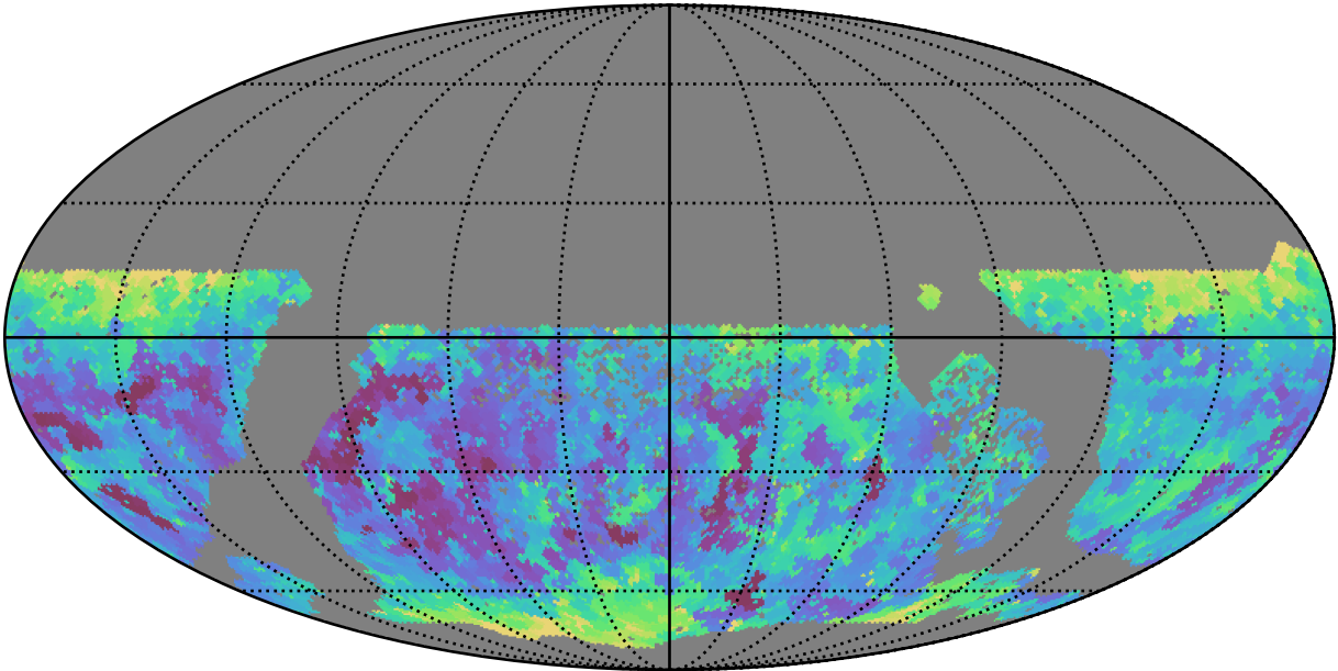
too_elab_r256_d2_griz_v3.4_10yrs WFD y band: Min seeingEff
