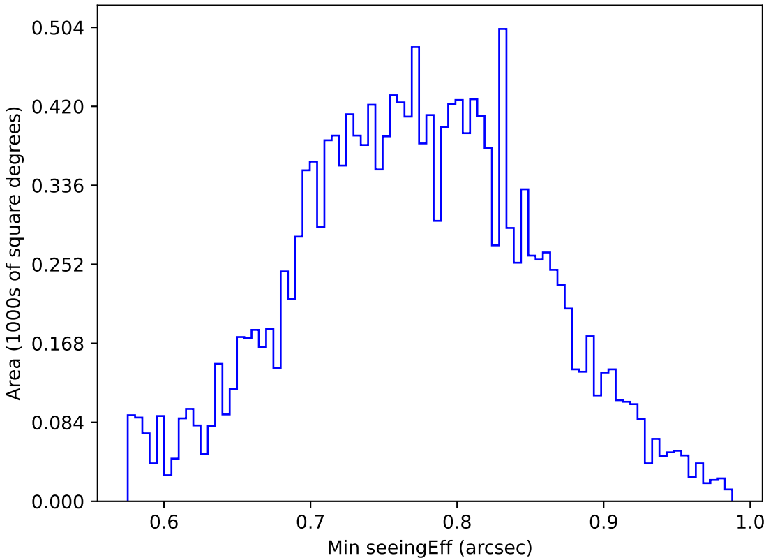
too_elab_r256_d2_griz_v3.4_10yrs WFD u band: Min seeingEff
