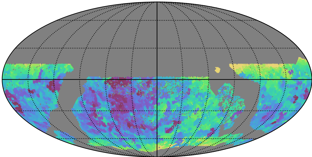
too_elab_r256_d2_griz_v3.4_10yrs WFD r band: Min seeingEff
