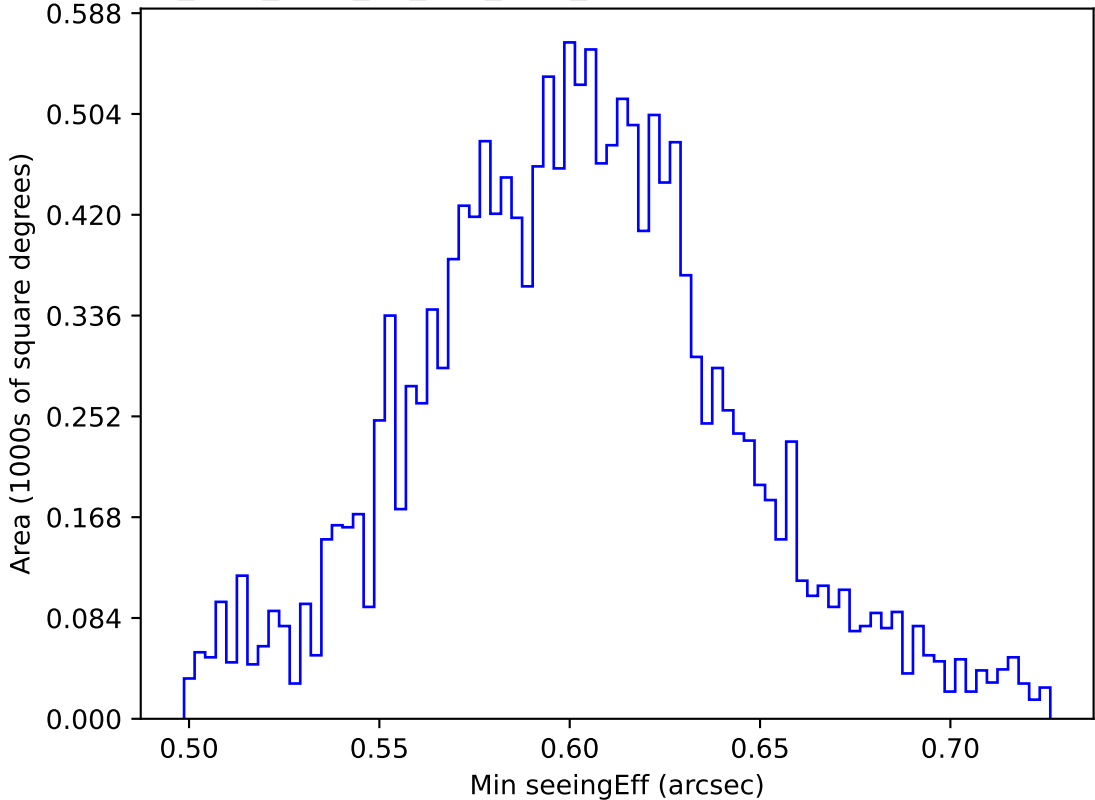
too_elab_r256_d2_griz_v3.4_10yrs WFD i band: Min seeingEff
