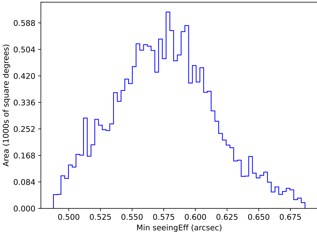
too_elab_r256_d2_griz_v3.4_10yrs WFD all bands: Min seeingEff
