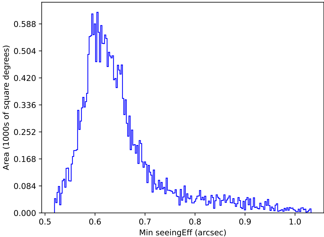
too_elab_r256_d2_griz_v3.4_10yrs All sky z band: Min seeingEff
