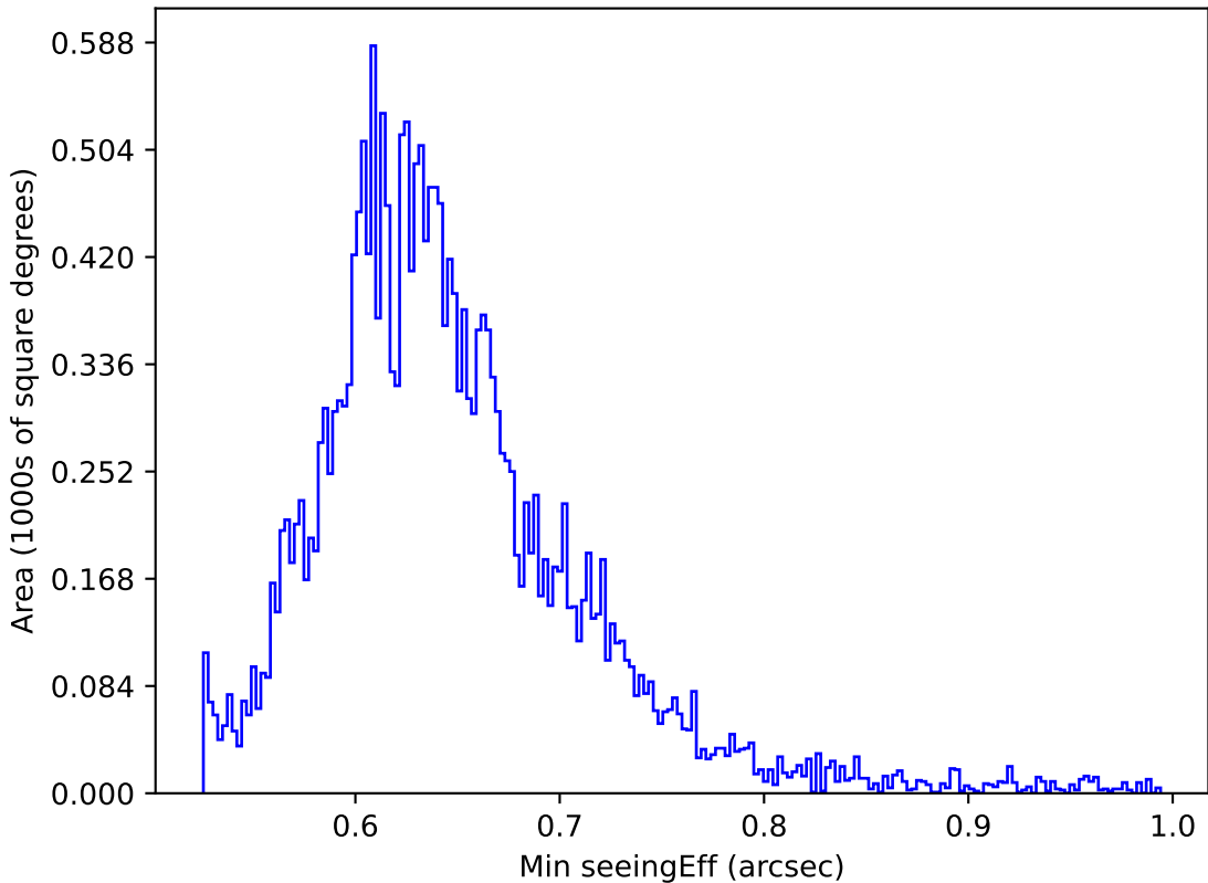
too_elab_r256_d2_griz_v3.4_10yrs All sky y band: Min seeingEff
