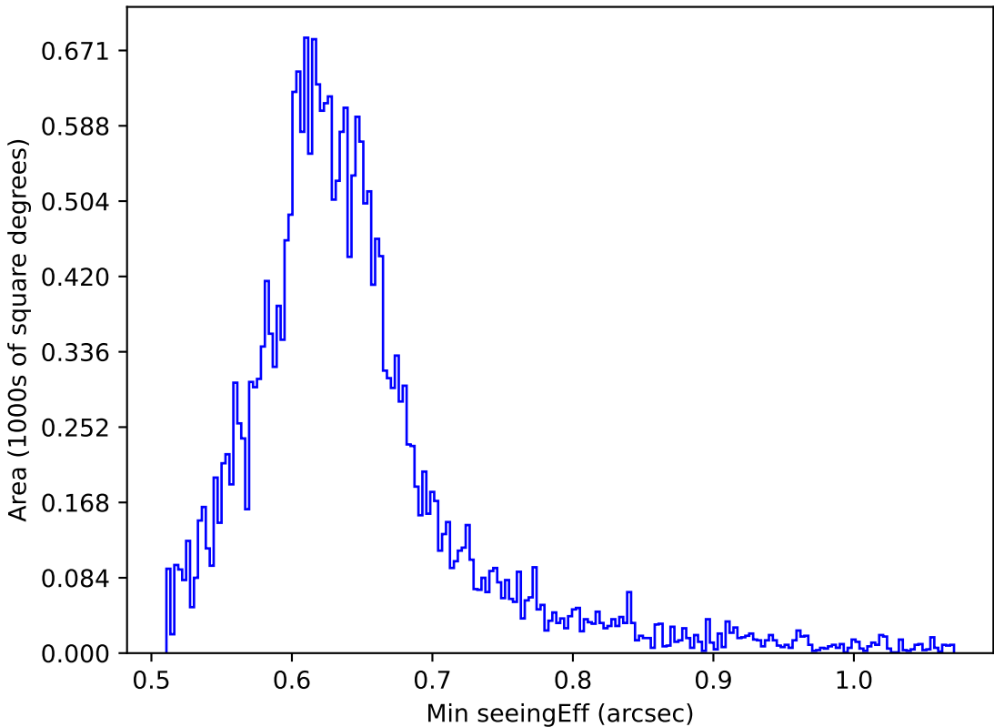
too_elab_r256_d2_griz_v3.4_10yrs All sky r band: Min seeingEff
