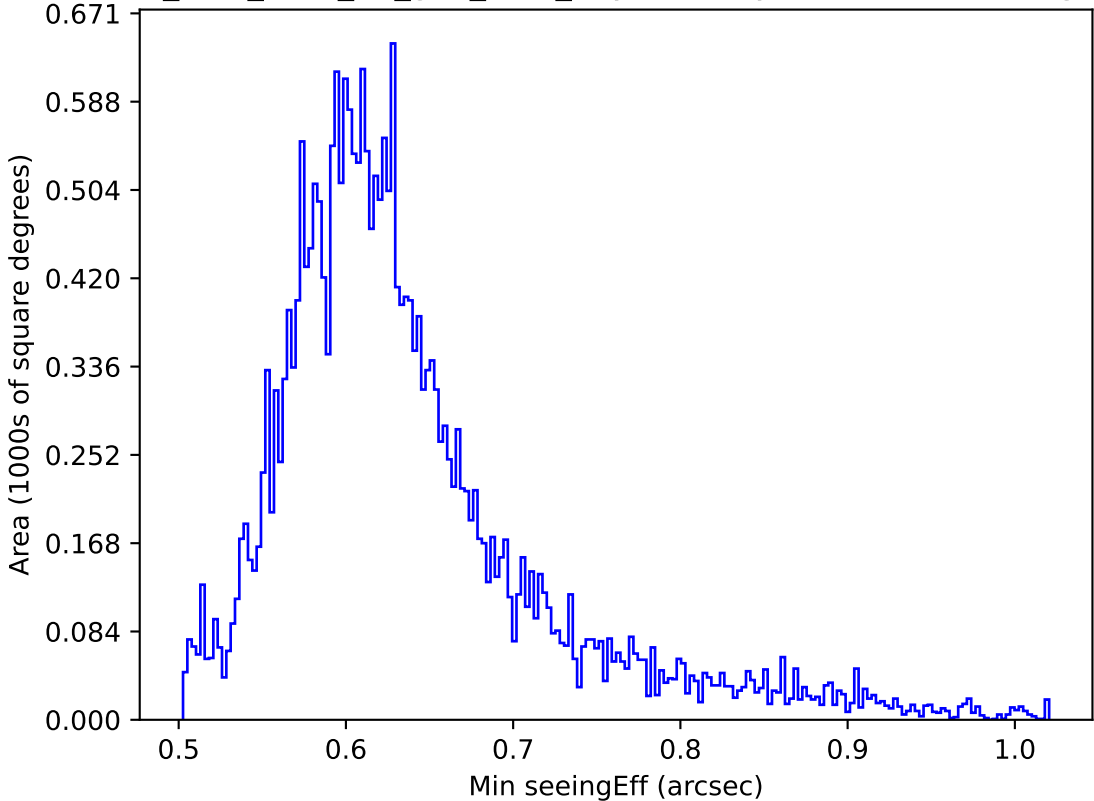
too_elab_r256_d2_griz_v3.4_10yrs All sky i band: Min seeingEff
