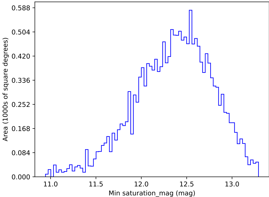
too_elab_r256_d2_griz_v3.4_10yrs WFD i band: Min saturation_mag
