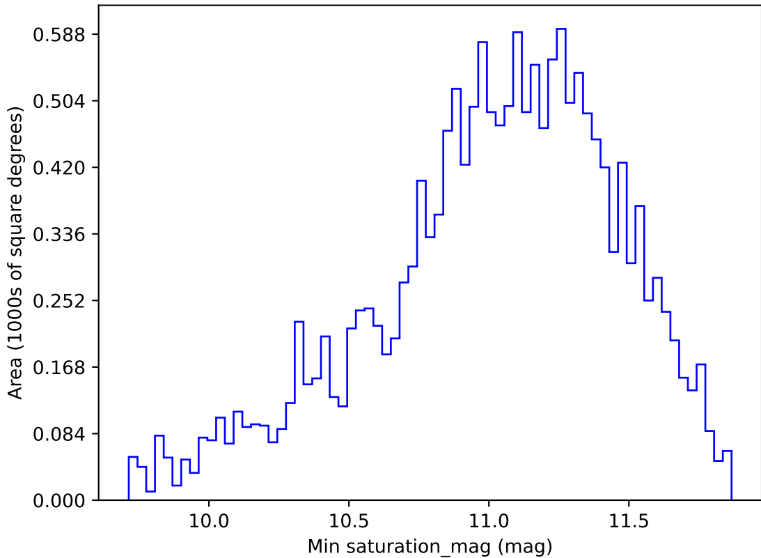
too_elab_r256_d2_griz_v3.4_10yrs WFD all bands: Min saturation_mag
