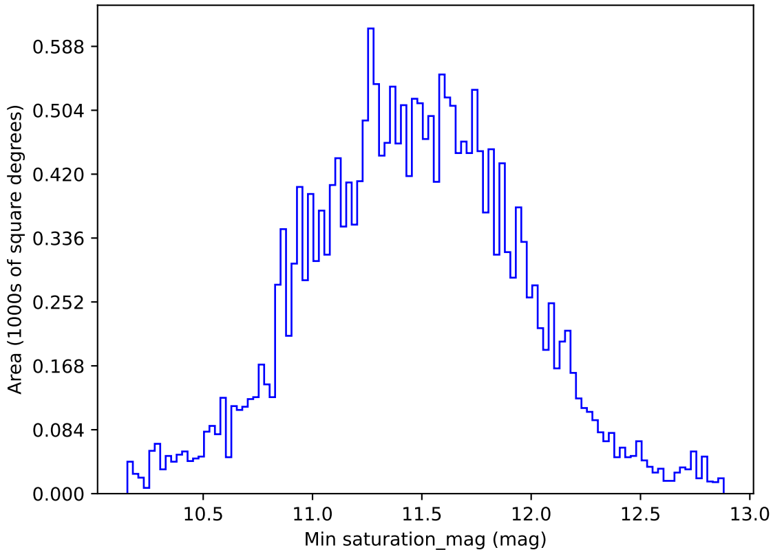
too_elab_r256_d2_griz_v3.4_10yrs All sky u band: Min saturation_mag
