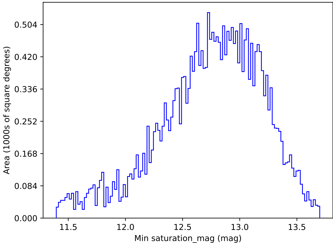
too_elab_r256_d2_griz_v3.4_10yrs All sky g band: Min saturation_mag
