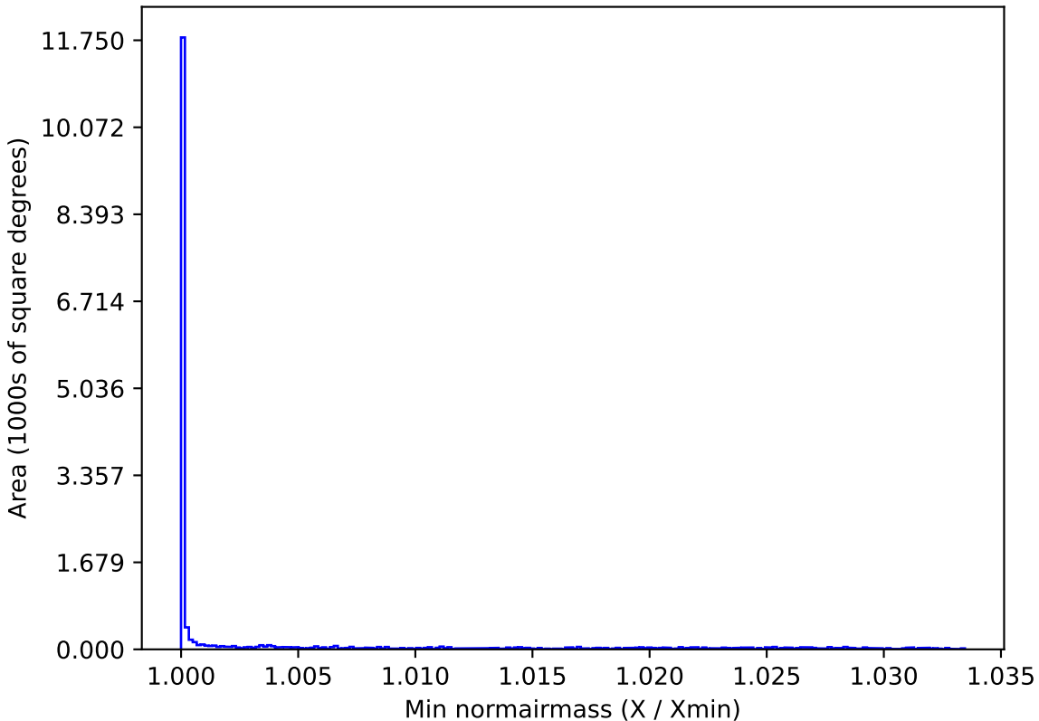
too_elab_r256_d2_griz_v3.4_10yrs WFD z band: Min normairmass
