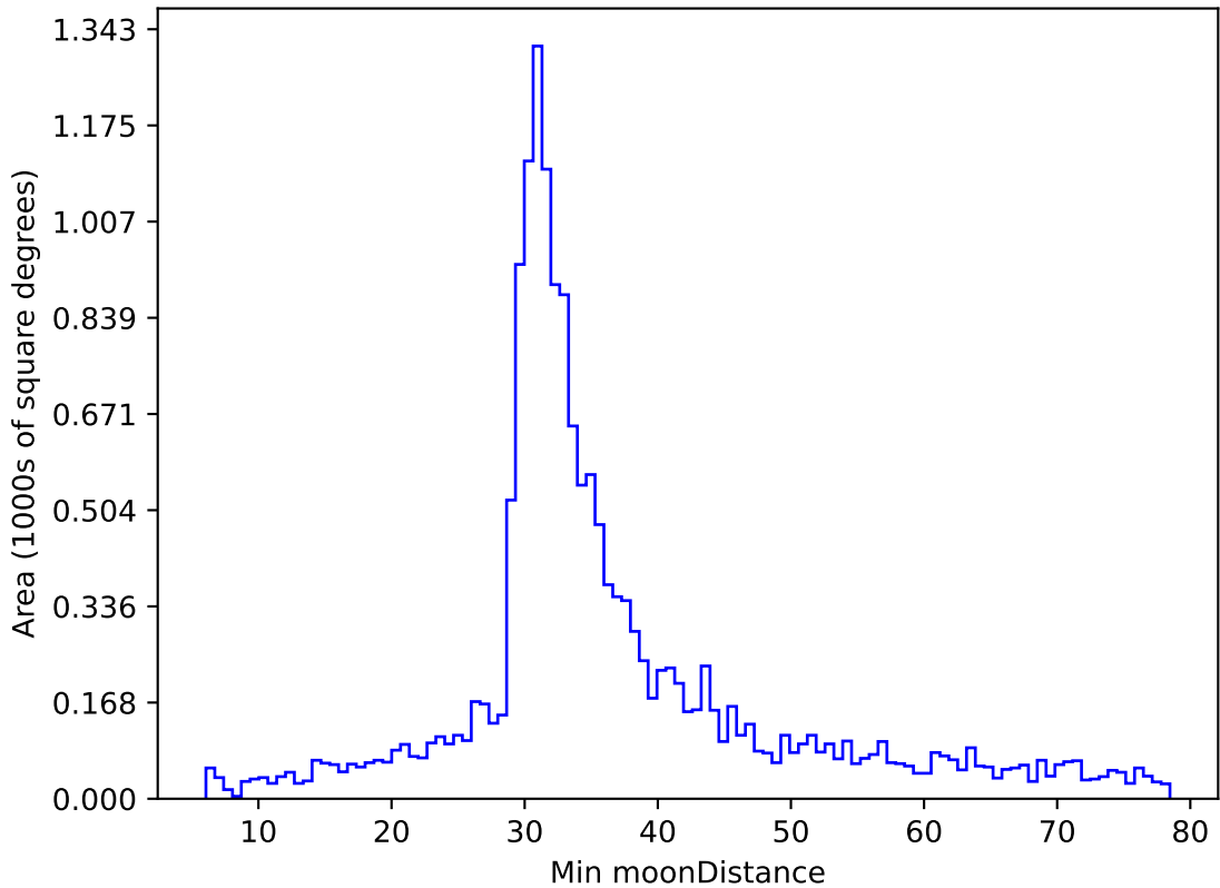
too_elab_r256_d2_griz_v3.4_10yrs WFD r band: Min moonDistance
