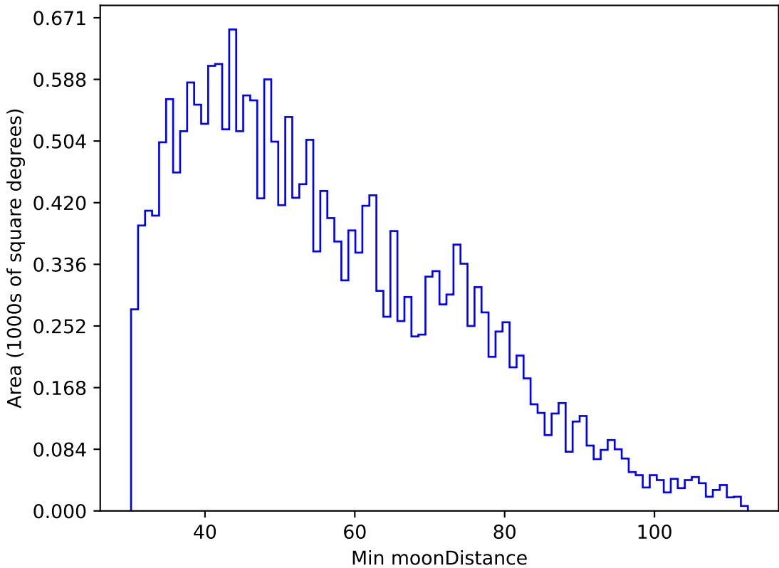
too_elab_r256_d2_griz_v3.4_10yrs All sky u band: Min moonDistance
