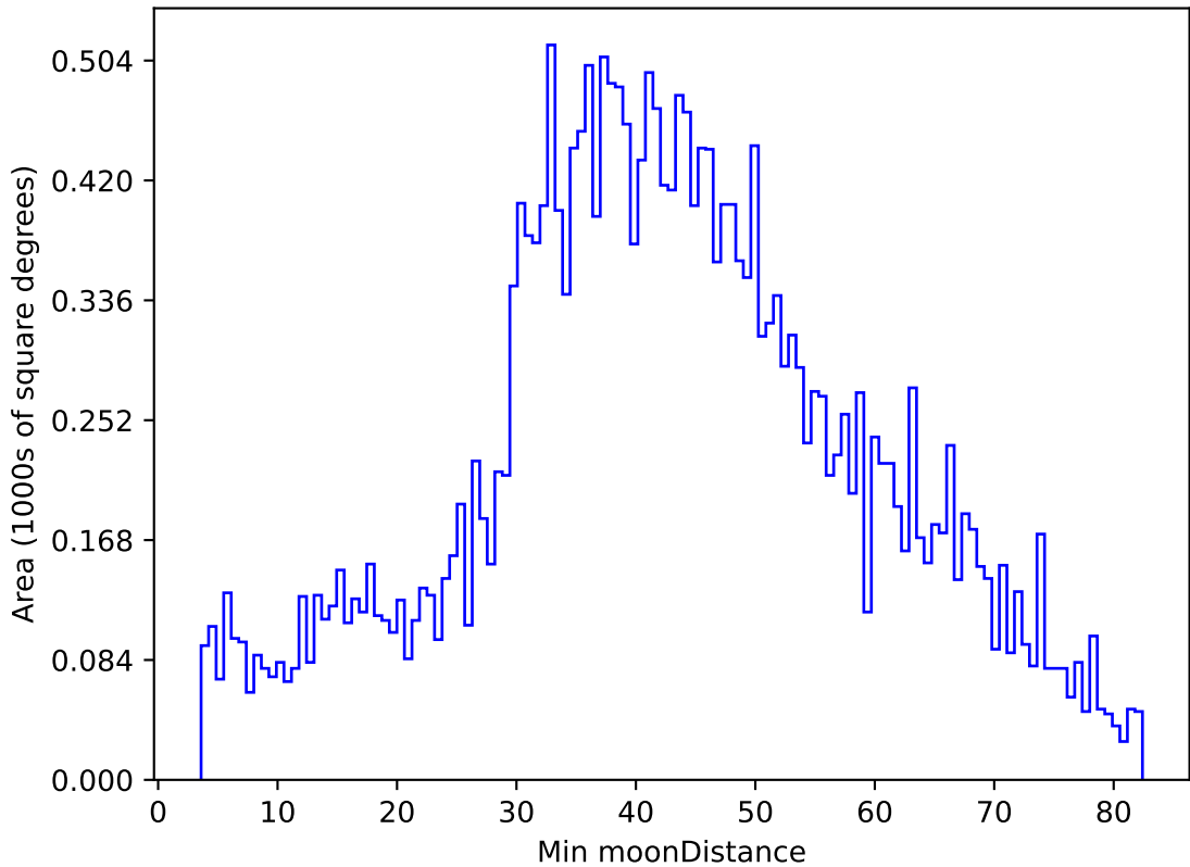
too_elab_r256_d2_griz_v3.4_10yrs All sky g band: Min moonDistance
