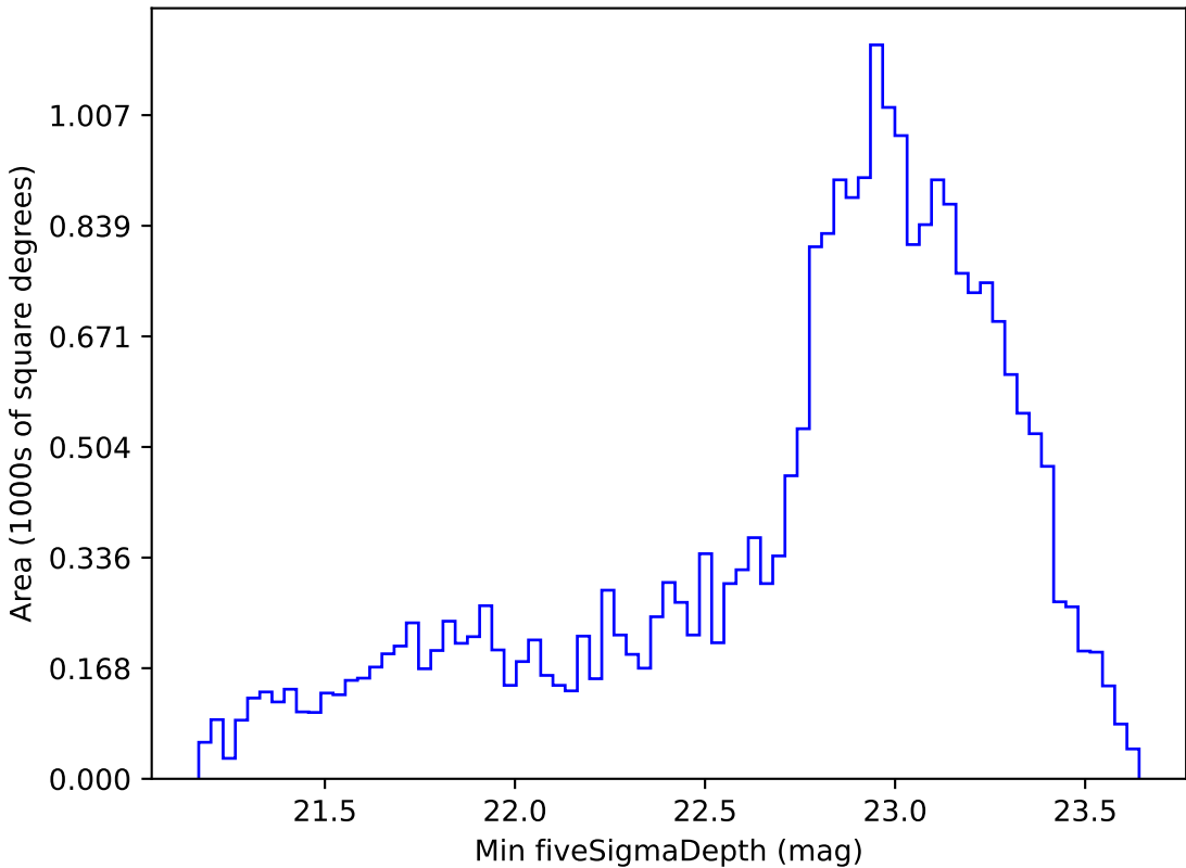
too_elab_r256_d2_griz_v3.4_10yrs Yr 1 i band: Min fiveSigmaDepth
