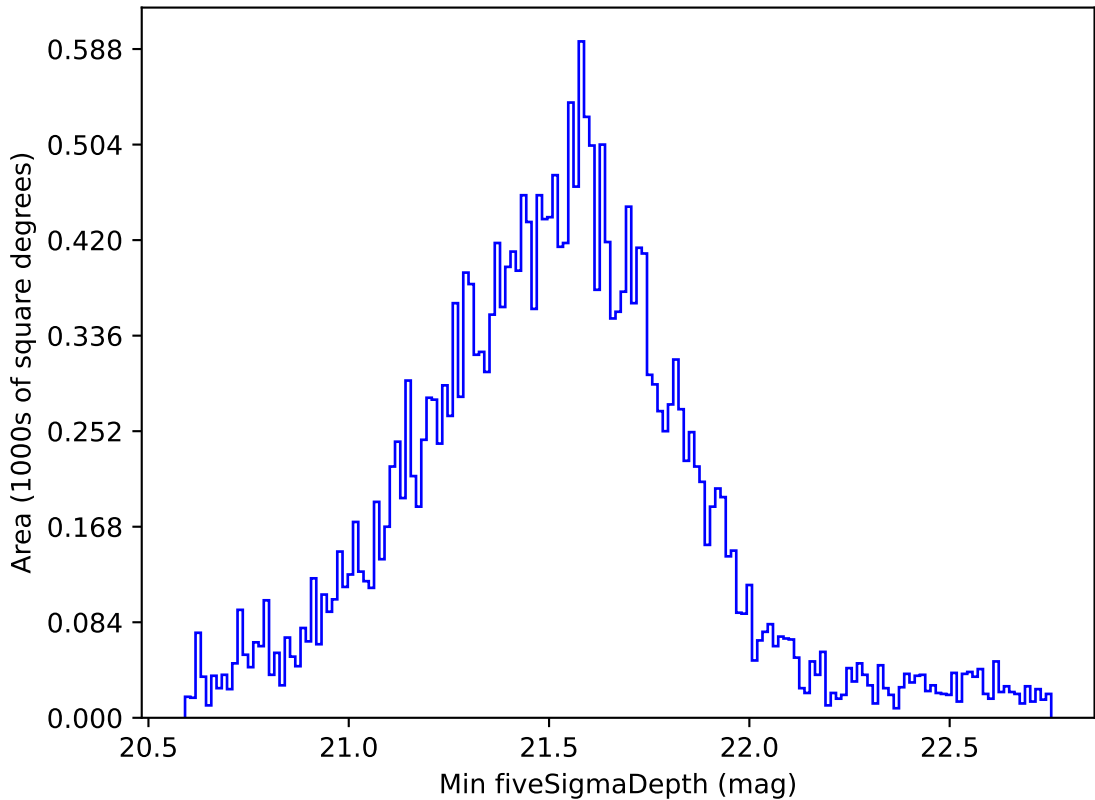
too_elab_r256_d2_griz_v3.4_10yrs Yr 1 all bands: Min fiveSigmaDepth
